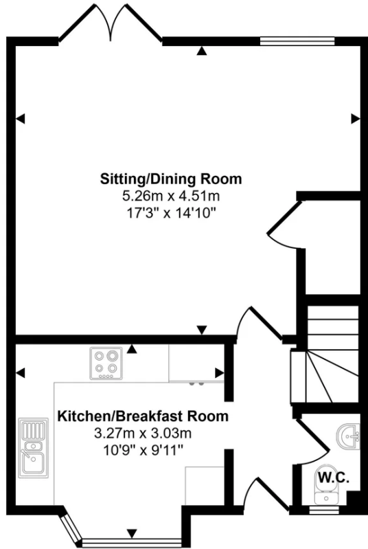
Ground Floor Approx 39 sq m / 419 sq ft
