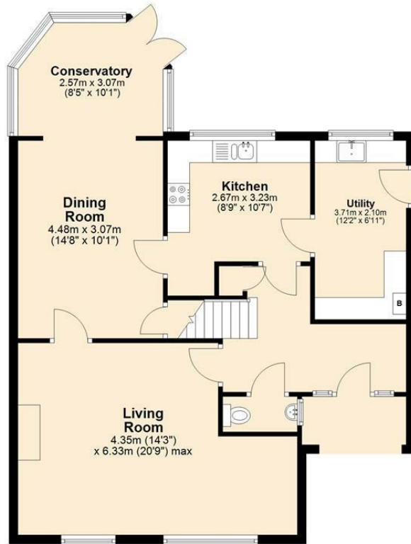
Ground Floor Approx. 80.0 sq. metres (861.6 sq. feet)
