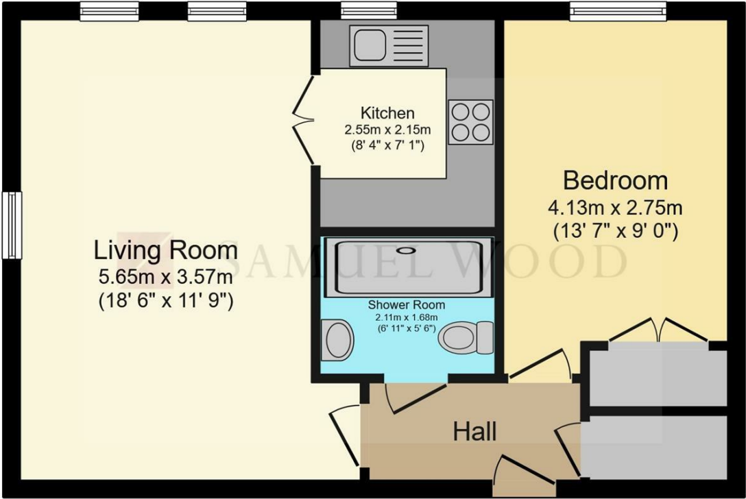
Floor Plan
