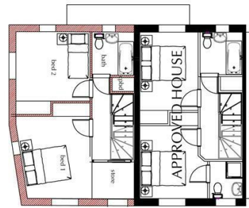
3b5p house First Floor Layout overall area 39 sq m storage area 3.7 sq m plus 2 sq m wardrobespace
