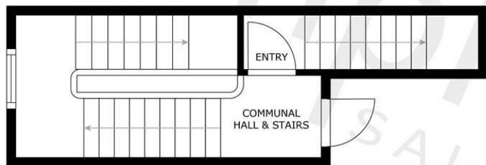
FLOOR 1
