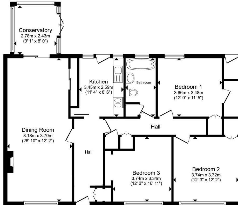
Floor Plan
