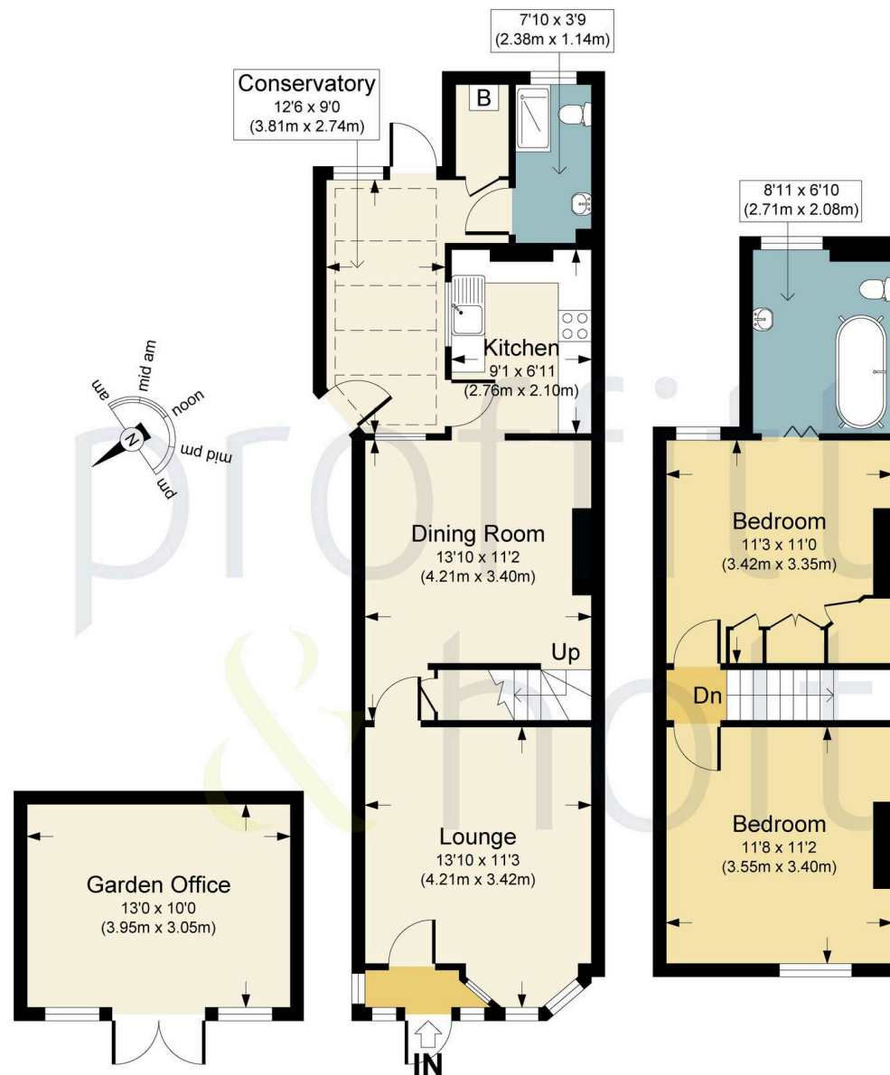
Ground Floor
