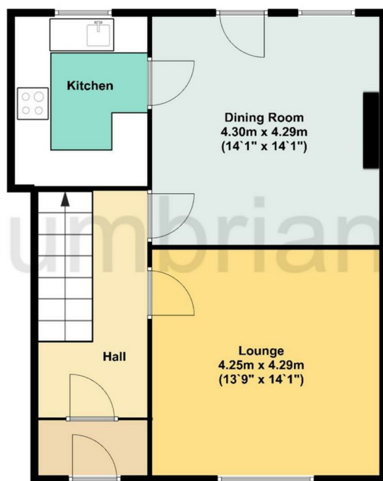
Ground Floor Approx 55.00 Sq meters (592.00 Sq feet).
