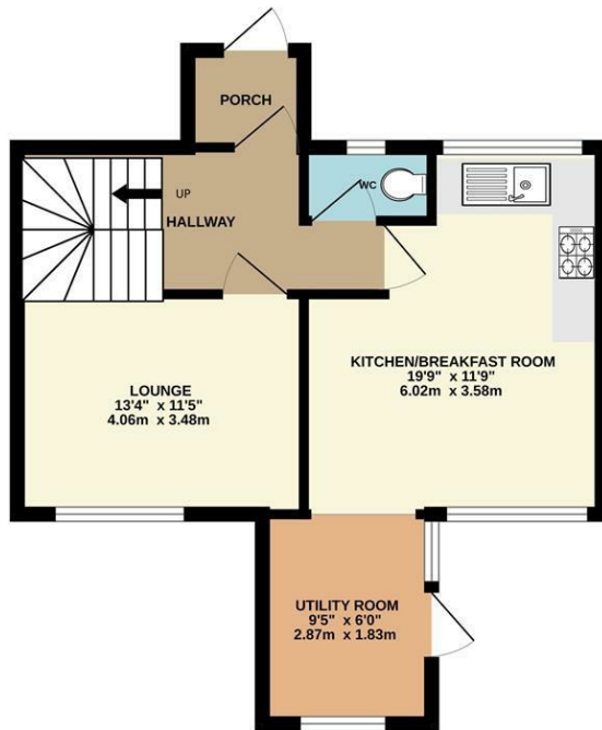
GROUND FLOOR 397 sq.ft. (36.9 sq.m.) approx.
