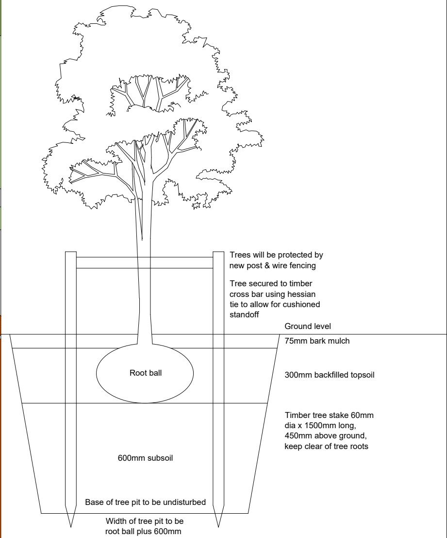
TREE PIT DETAIL 1:20
